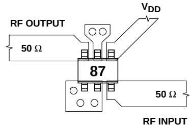
Figure 14. RF Layout.
