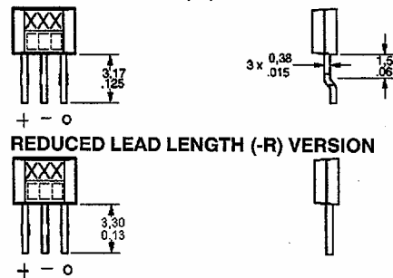
SURFACE MOUNT (-S) VERSION
