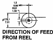
REDUCED LEAD LENGTH (-R) VERSION
