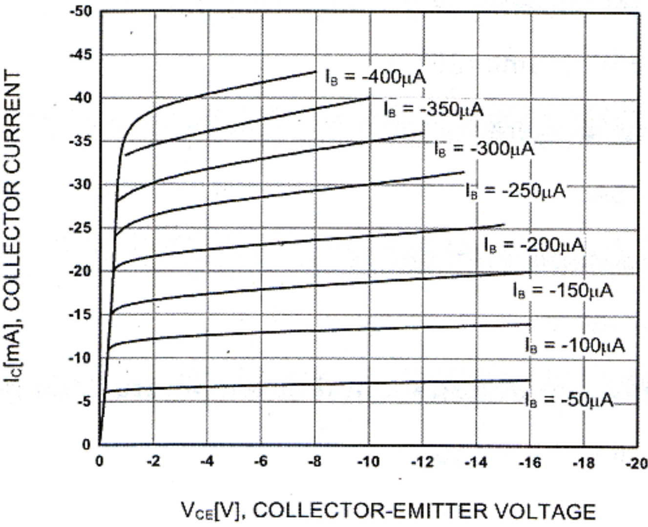
Static Characteristic
