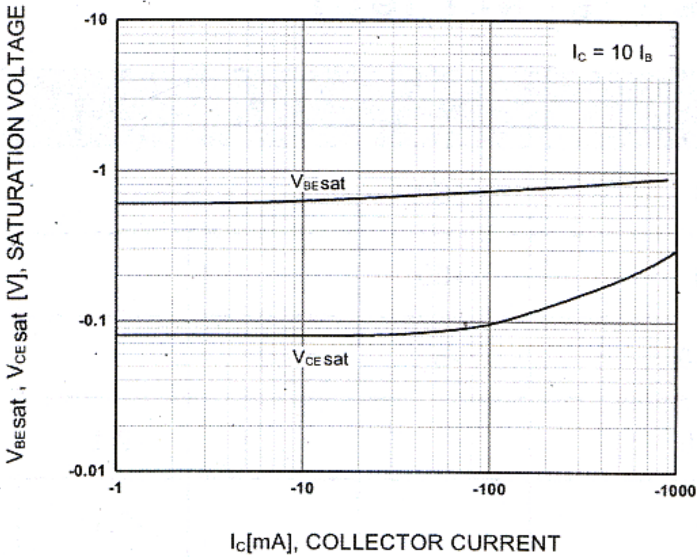
Base-Emitter Saturation Voltage Collector-Emitter Saturation Voltage
