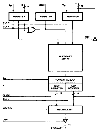
Am29516/29516A/29L516
