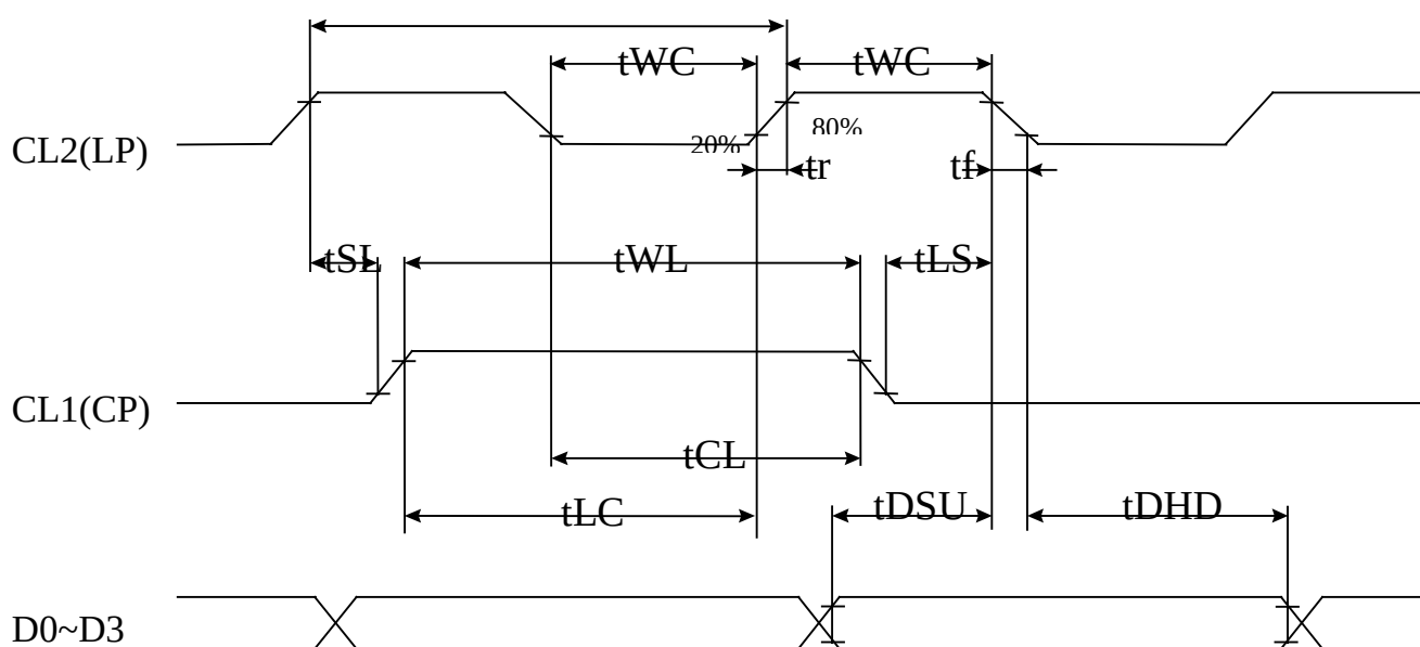
Fig 1. SEGMENT TIMING
