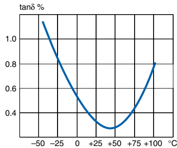
Dissipation factor vs. temperature
