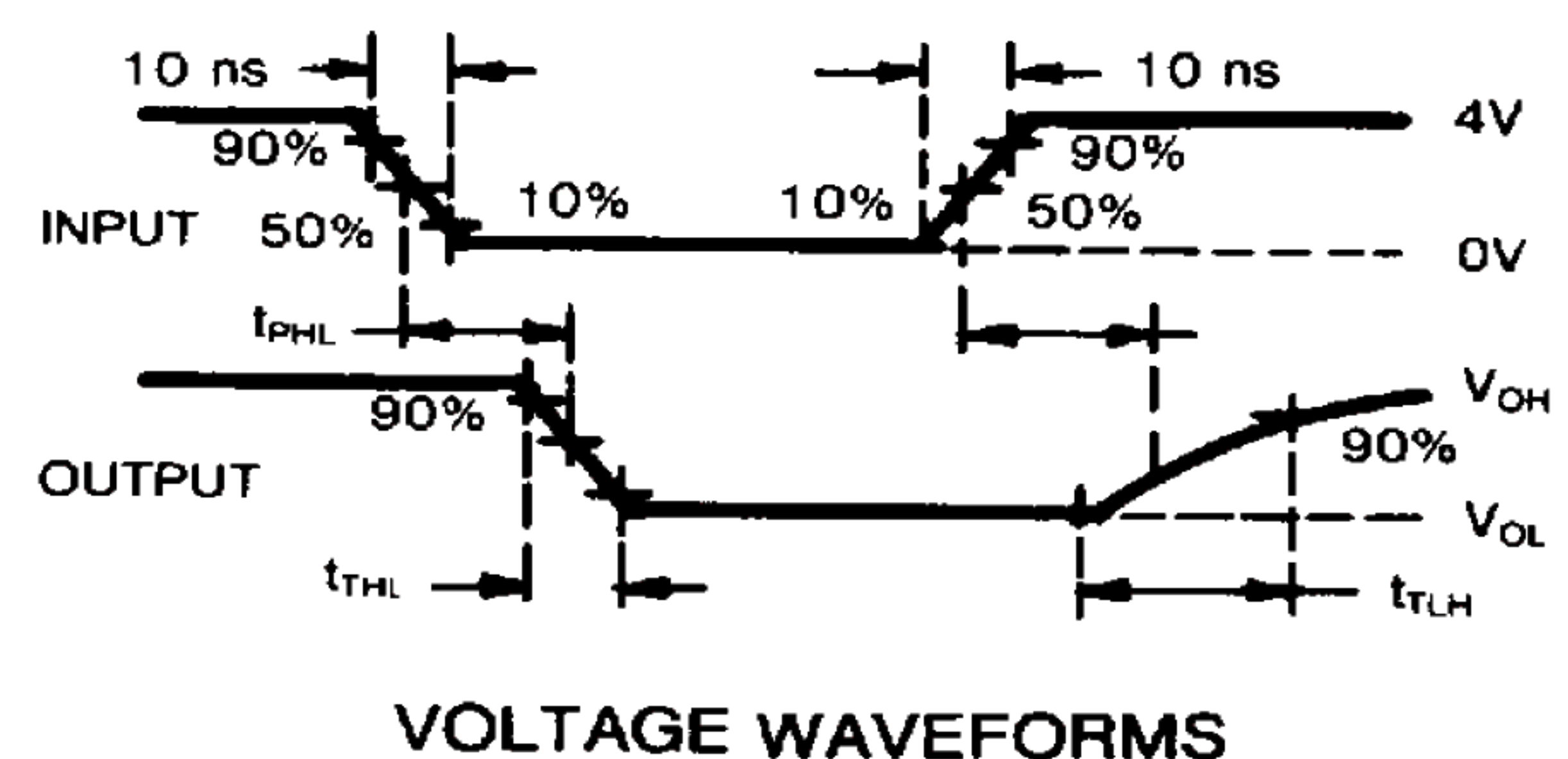
Figure 4 - Switching Times
