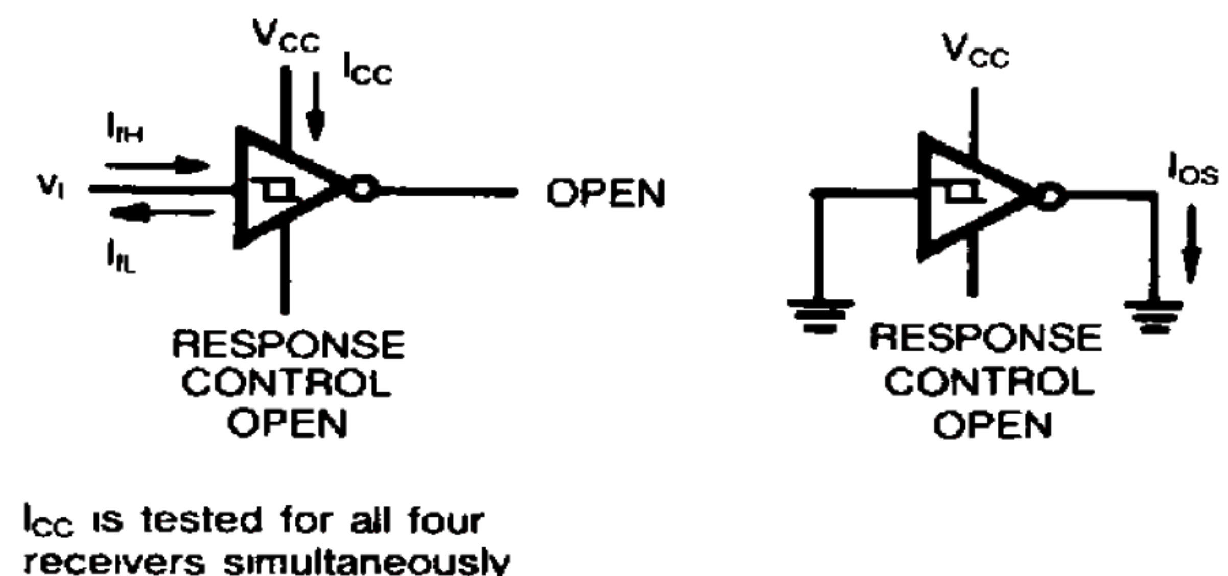
Figure 2 — I_{IH} , I_{IL} , I_{CC}
