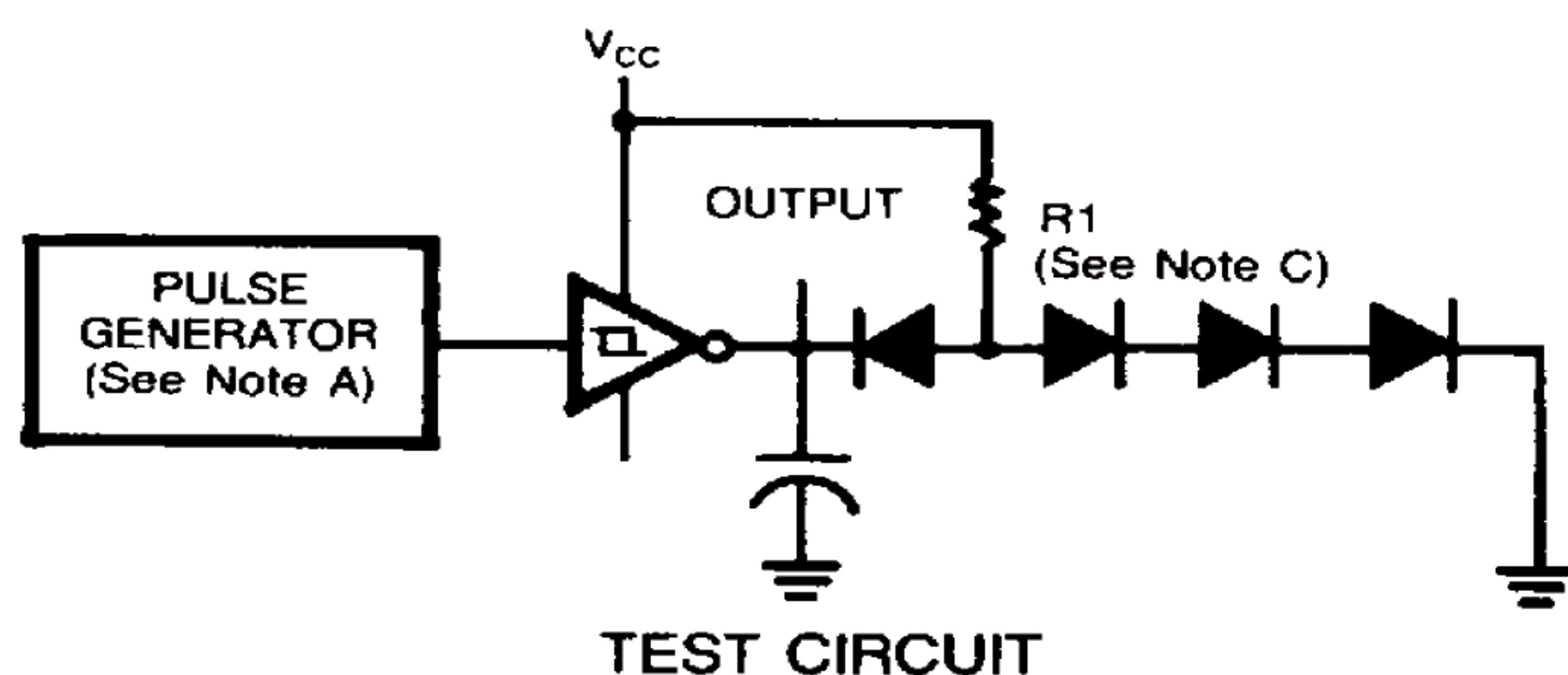
Figure 4 - Switching Times
