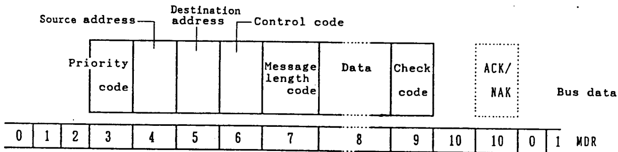
Figure 3.9 ACK/NAK error
