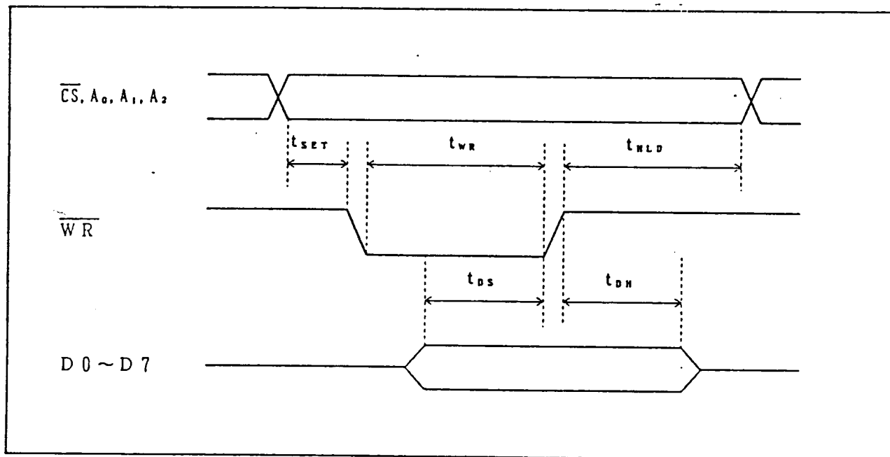
Figure 5.4 Write timing
