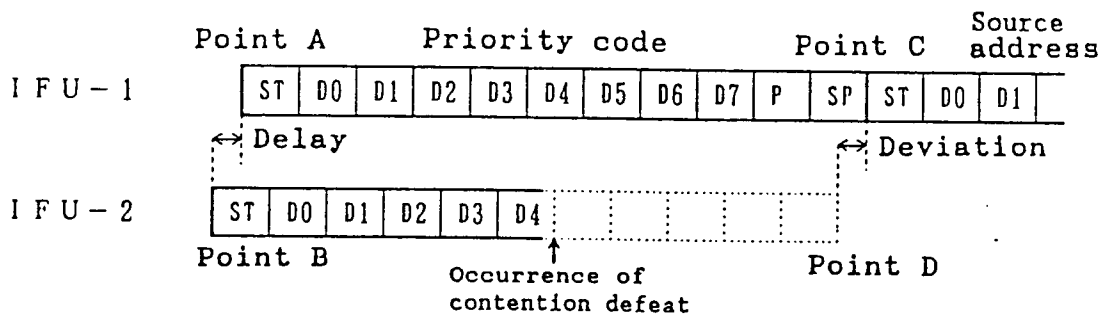
Figure 3.4 "Deviation" in contention
