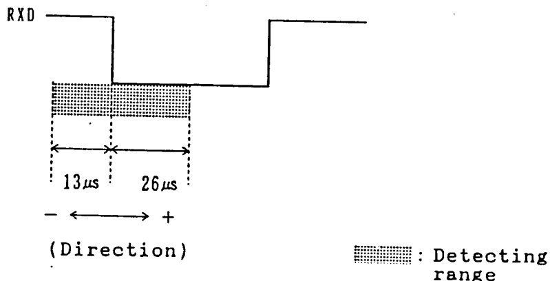
Figure 3.3 Start bit position detect range (for ② through ⑧ in Figure 3.2)
