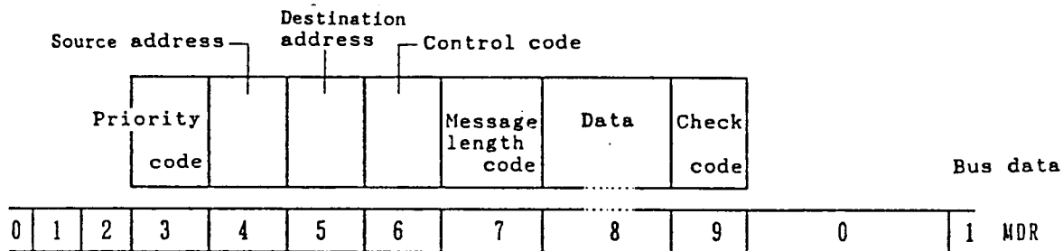
Figure 3.7 Broadcasting packet
