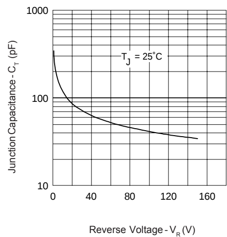
Fig. 3 - Typical Junction Capacitance Vs. Reverse Voltage
