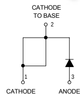
TO-247AC (Modified)
