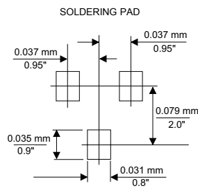
Outline SOT23
