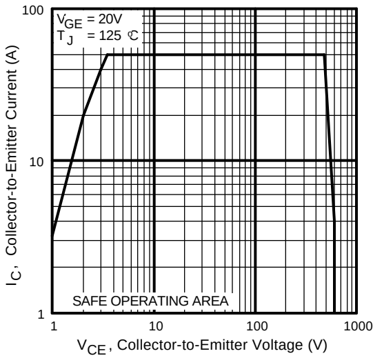
Fig. 12 - Turn-Off SOA
