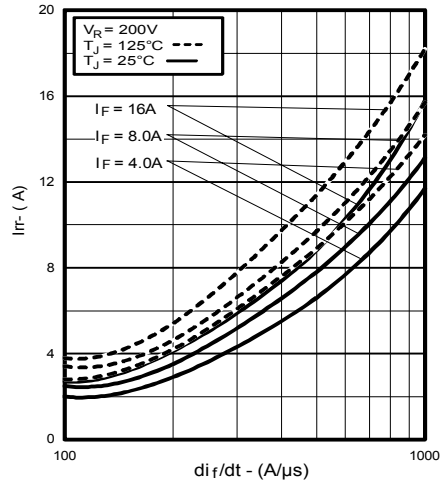
Fig. 6 - Typical Recovery Current vs. di/dt , (per Leg)
