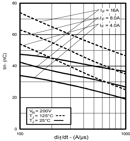
Fig. 5 - Typical Reverse Recovery vs. di/dt , (per Leg)
