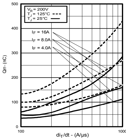
Fig. 7 - Typical Stored Charge vs. di/dt , (per Leg)
