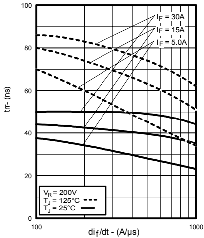
Fig. 5 - Typical Reverse Recovery Time vs. di/dt
