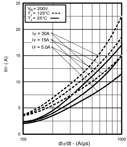
Fig. 6 - Typical Recovery Current vs. di_T/dt , (per Leg)
