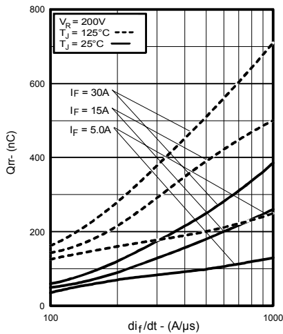
Fig. 7 - Typical Stored Charge vs. di_T/dt , (per Leg)
