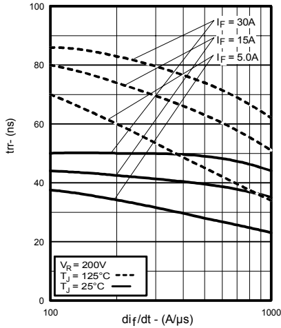
Fig. 5 - Typical Reverse Recovery Time vs. di_T/dt , (per Leg)
