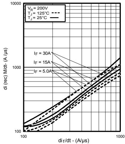
Fig. 8 - Typical di_{(rec)}M/dt vs. di_T/dt , (per Leg)
