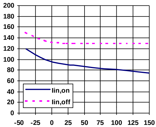
Figure 17 - Input current (μA) Vs Tj (°C)
