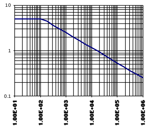
Figure 10 - Max. I_{out} (A) Vs Load Inductance (uH)
