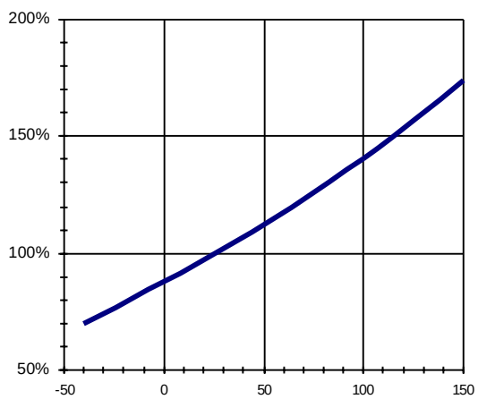
Figure 8 - Normalized R_{ds(on)} (m \Omega ) Vs T_j ( ^{\circ} C)
