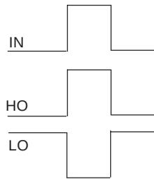
Figure 1. Input/Output Timing Diagram
