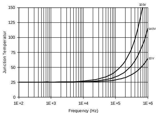
Figure 29. IR2110 T_J vs. Frequency (IRFBC30) R_{GATE} = 22\Omega , V_{CC} = 15V
