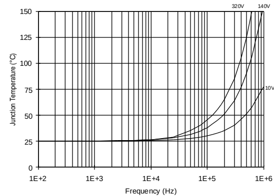
Figure 32. IR2110L6S T_J vs. Frequency (IRFBC20) R_{GATE} = 33W , V_{CC} = 15V
