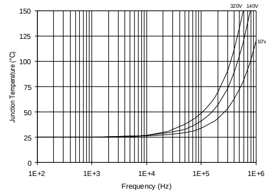
Figure 34. IR2110L6S T_J vs. Frequency (IRFBC40) R_{GATE} = 15W , V_{CC} = 15V
