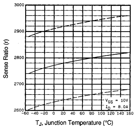
Fig 15. Typical HEXSense Ratio Vs. Junction Temperature
