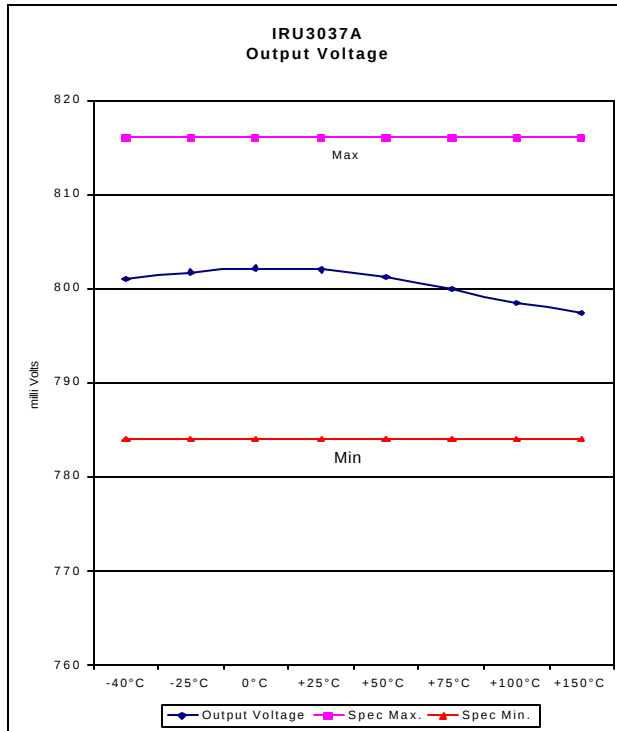
Figure 14 - Output Voltage
