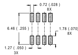
RECOMMENDED FOOTPRINT
