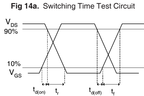
Fig 14b. Switching Time Waveforms www.irf.com
