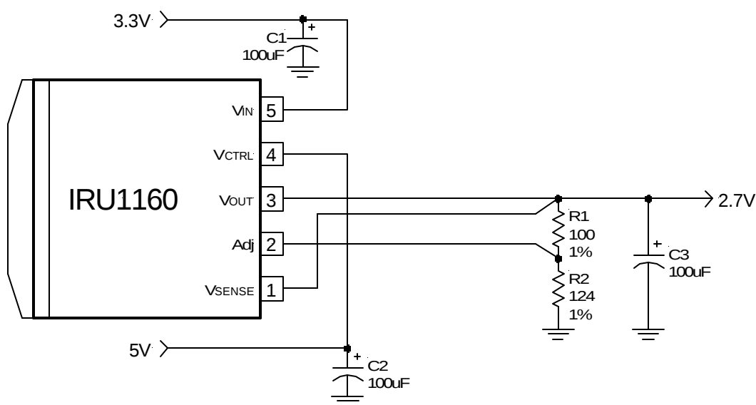
Figure 1 - Typical application of IRU1160 in a 3.3V to 2.8V.
