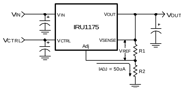
Figure 3 - Typical application of the IRU1175 for programming the output voltage.
