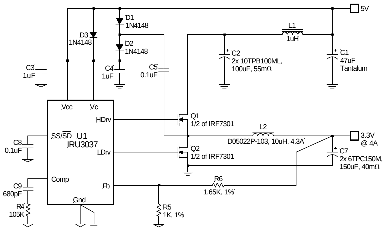
Figure 18 - Typical application of IRU3037 in an on-board DC-DC converter using a single 5V supply.
