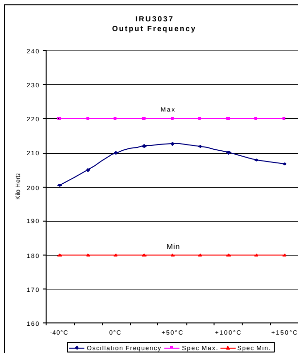
Figure 12 - Output Frequency
