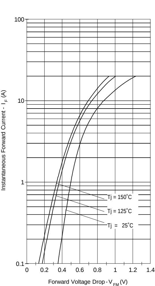
Fig. 1 - Max. Forward Voltage Drop Characteristics
