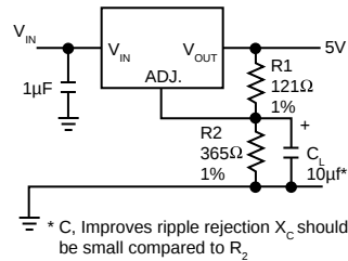
Improving Ripple Rejection
