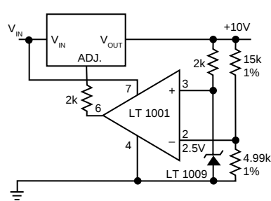
Precision High Current Reference
