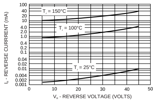
TYPICAL REVERSE CURRENT OM4213SC
