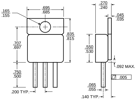
MECHANICAL OUTLINE
