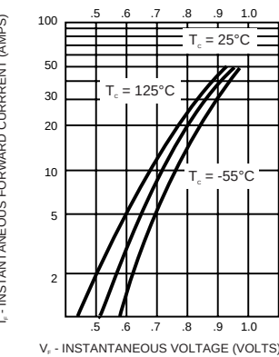
TYPICAL FORWARD VOLTAGE OM4220SC
