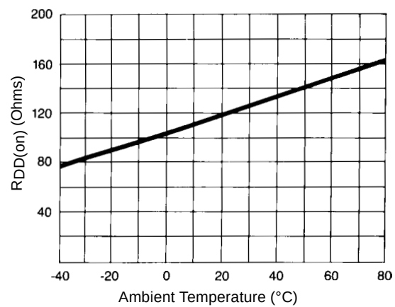
Figure 4. Typical On-Resistance
