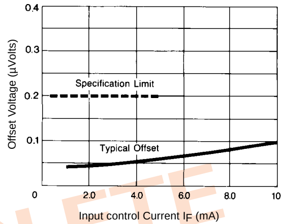
Figure 2. Offset Voltage
