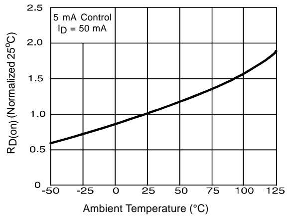
Figure 4. Typical On-Resistance
