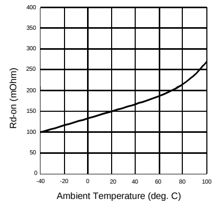
Figure 4. Typical On-Resistance
