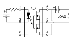
"C" Connection
