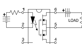
"B" Connection
