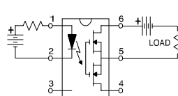
"B" Connection
