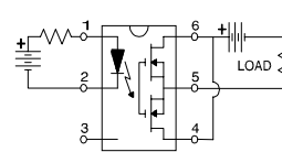
"C" Connection
