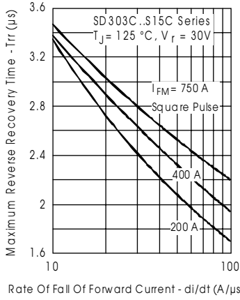
Fig. 15 - Recovery Time Characteristics
