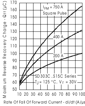
Fig. 16 - Recovery Charge Characteristics
