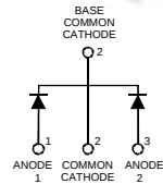
TO-220
