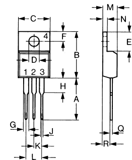
TO-220 AB Outline
