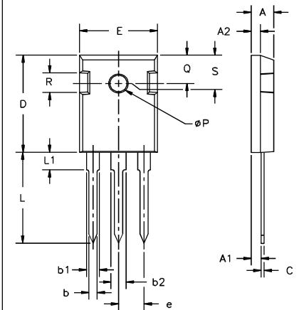
TO-247 AD Outline
