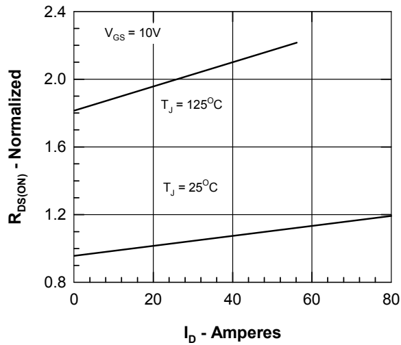
Figure 3. R_{DS(on)} normalized to 0.5 I_{D25} value vs. I_D
