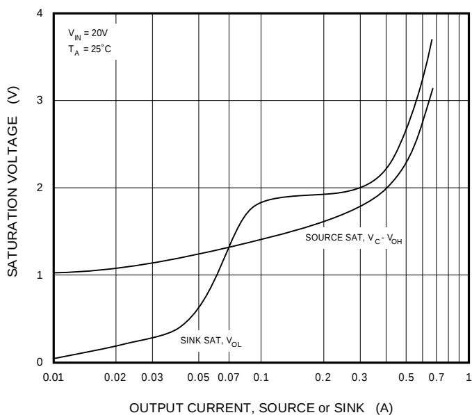
IP1525A Output Saturation Characteristics
