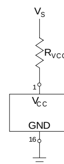
Current Fed Dropping Resistor
