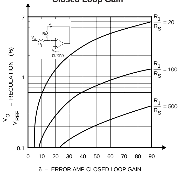
Regulation vs Error Amp Closed Loop Gain
