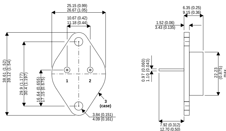
TO-3 Package Pin 1 – Gate Pin 2 – Source Pin 3 – Drain
