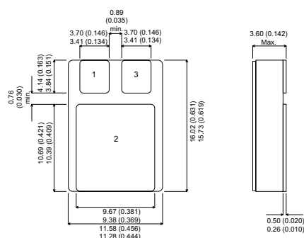
SMD1 Pin 1 – Gate Pin 2 – Source Pin 3 – Drain
