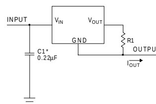
Current Regulator
