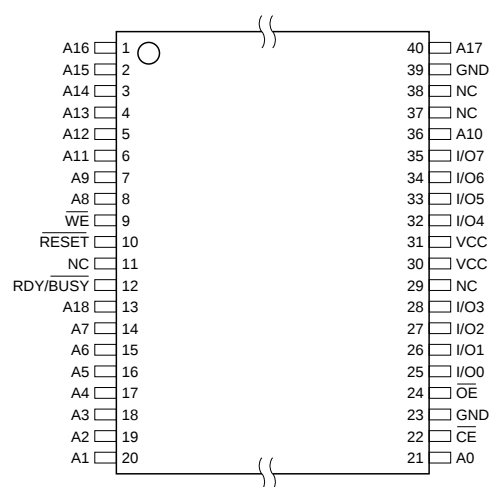
AT49F004(T) TSOP Top View Type 1
