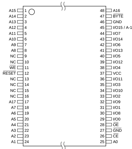
AT49F4096A(T) TSOP Top View Type 1
