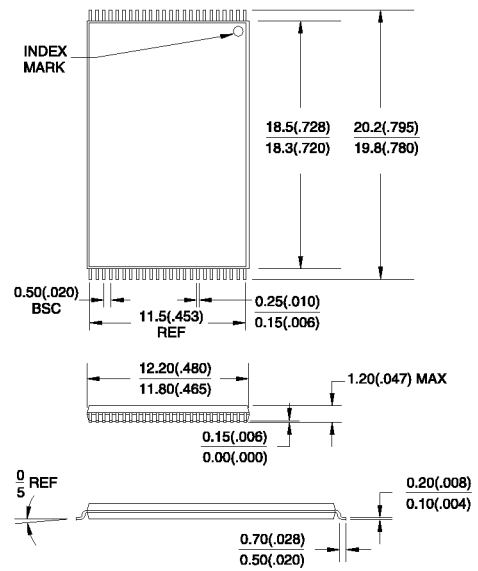
48T, 48-Lead, Plastic Thin Small Outline Package (TSOP) Dimensions in Millimeters and (Inches)* JEDEC OUTLINE MO-142 D
