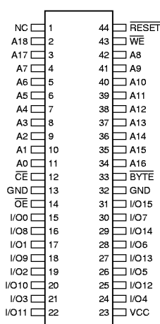
AT49F8192A(T) SOIC (SOP) Top View
