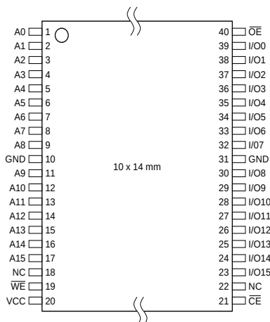
AT49F1025 VSOP Top View
