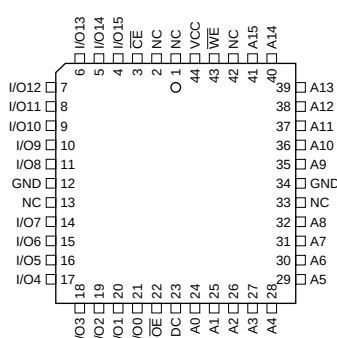
PLCC Top View
