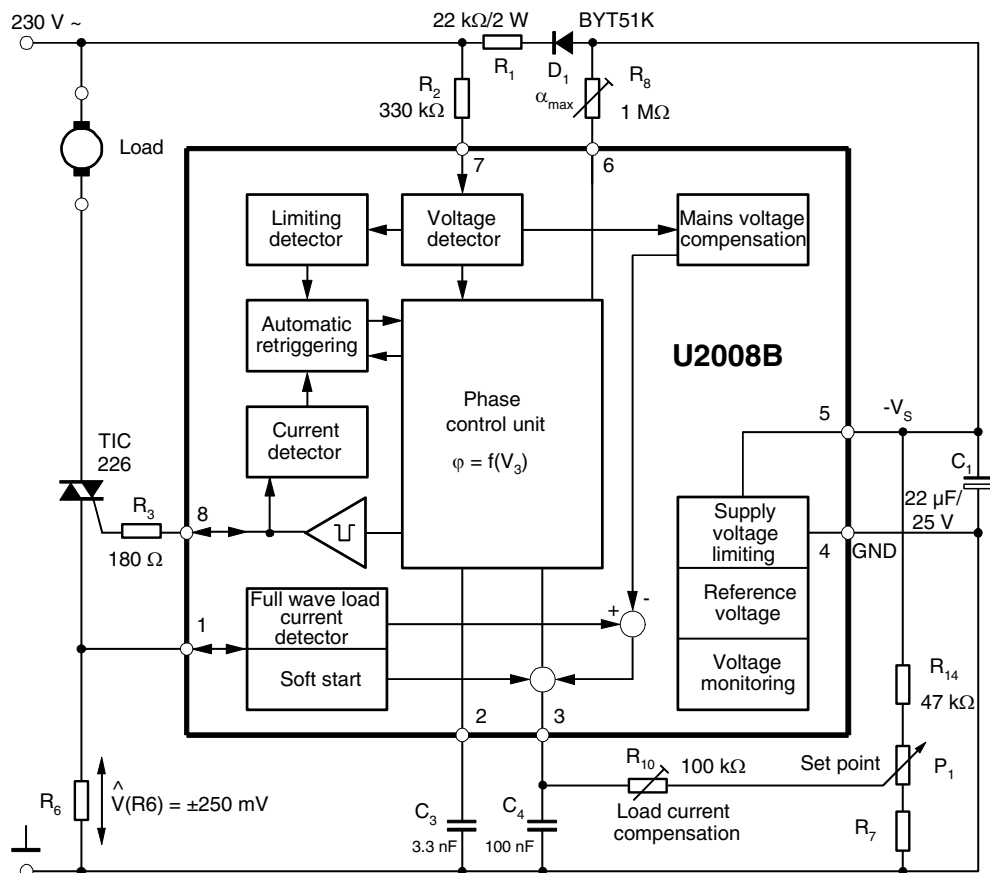
Figure 1. Block Diagram with Typical Circuit: Load Current Sensing
