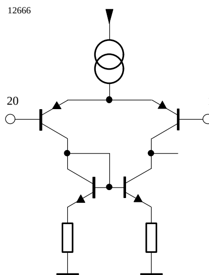
Figure 19. Pin 20 OP_{in-}
