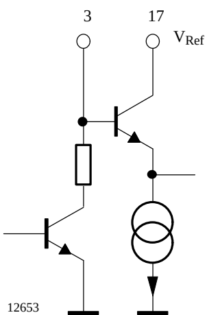
Figure 6. Pin 3 RC_{wake}
